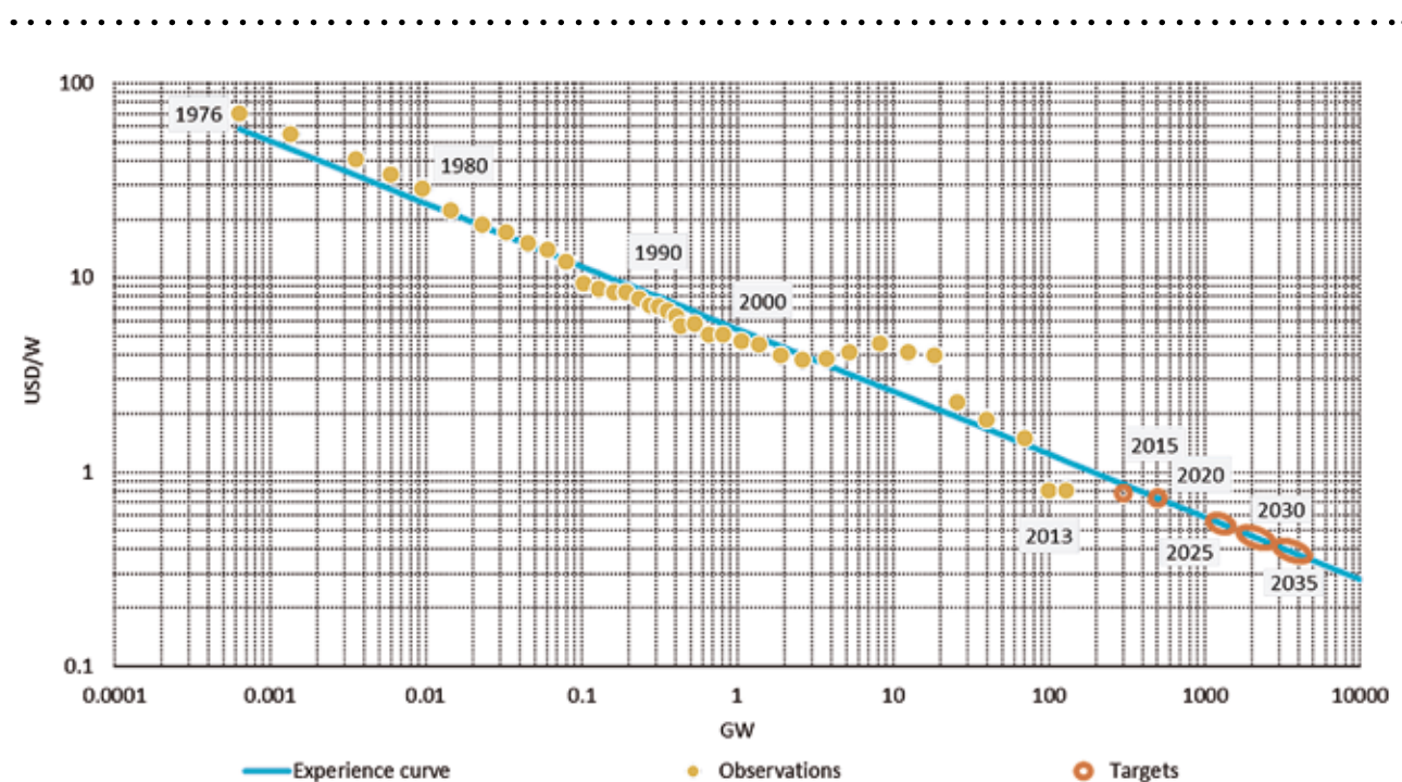
Figure 3-12 | Declining prices for crystalline modules (IEA)
