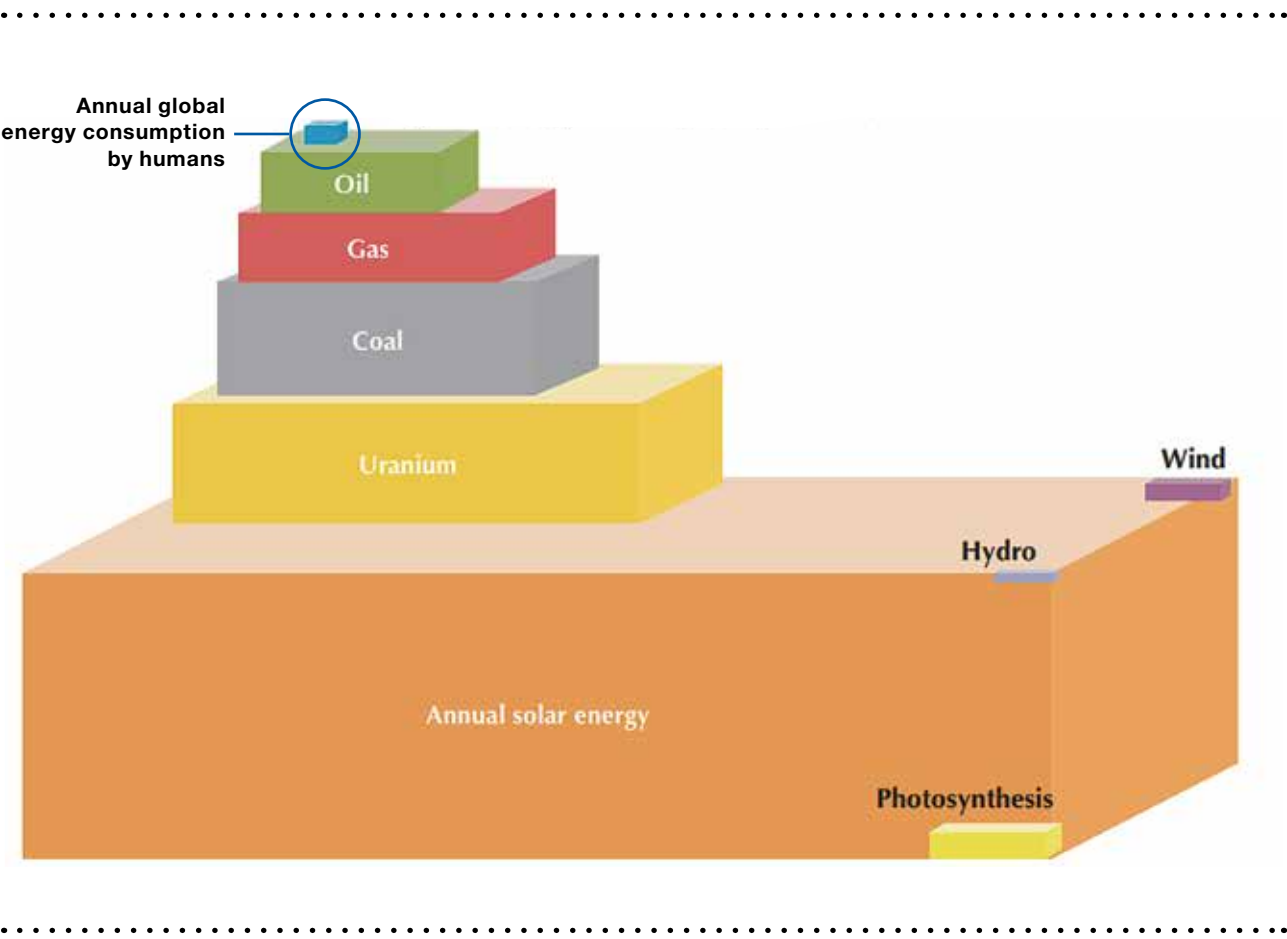
Figure 3-4 | Annual global energy consumption by humans set against known resources (IEA 2012)
